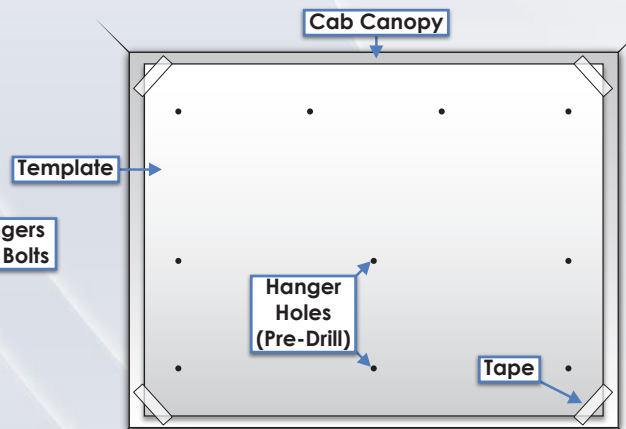
Figure 2: Cab Canopy (looking up)
